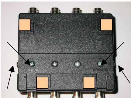
BOTTOM VIEW WITH 4 GROUNDING LOCATIONS & 4 RUBBER FEET AREAS
