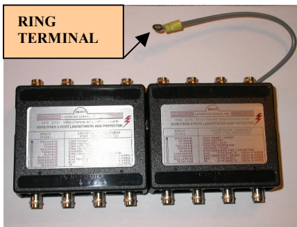
TOP VIEW WITH HORIZONTAL STACKING & 12 AWG GROUND WIRE
